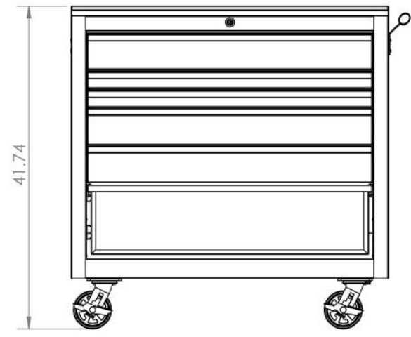
EX4106TC-00 (SCHEMATIC)
